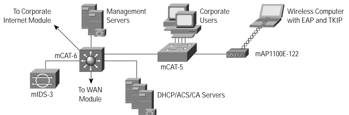
Figure A-17 Medium-Enterprise EAP WLAN Design
